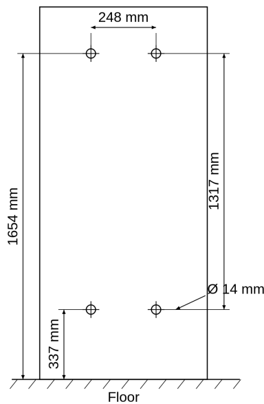
Wall view – position of the four drilling holes. Drawing not to scale.
